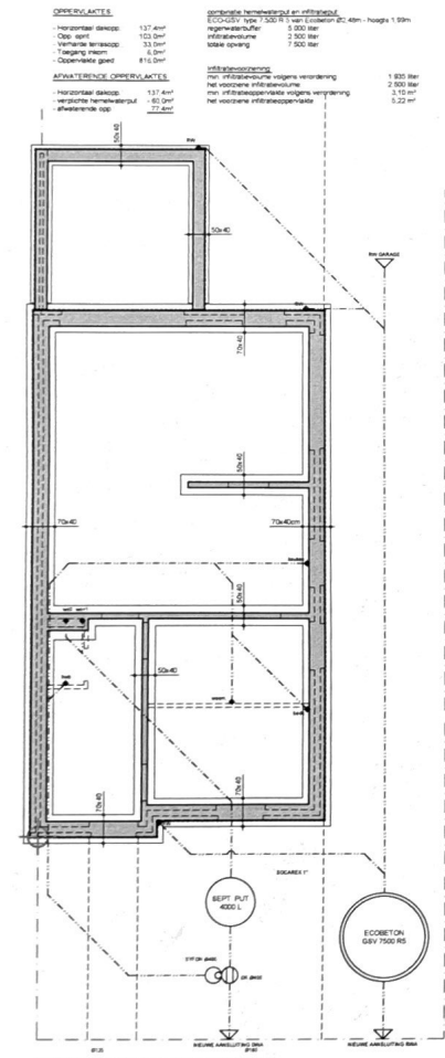
FUNDERING+RIOLERING
