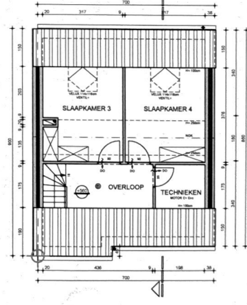
ZOLDER
