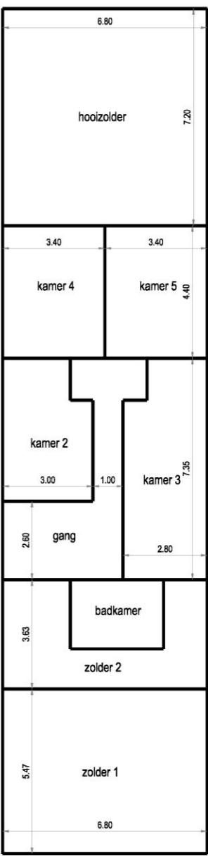
ZOLDERVERDIEPING
