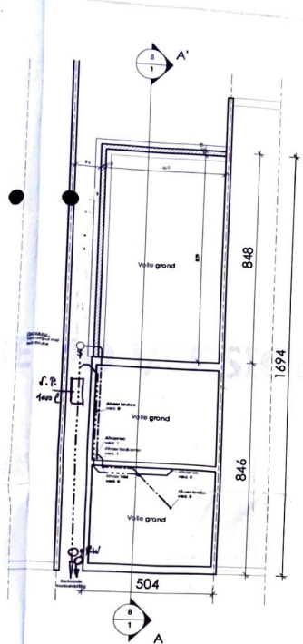
Funderingsplan/ Rioleringsplan
