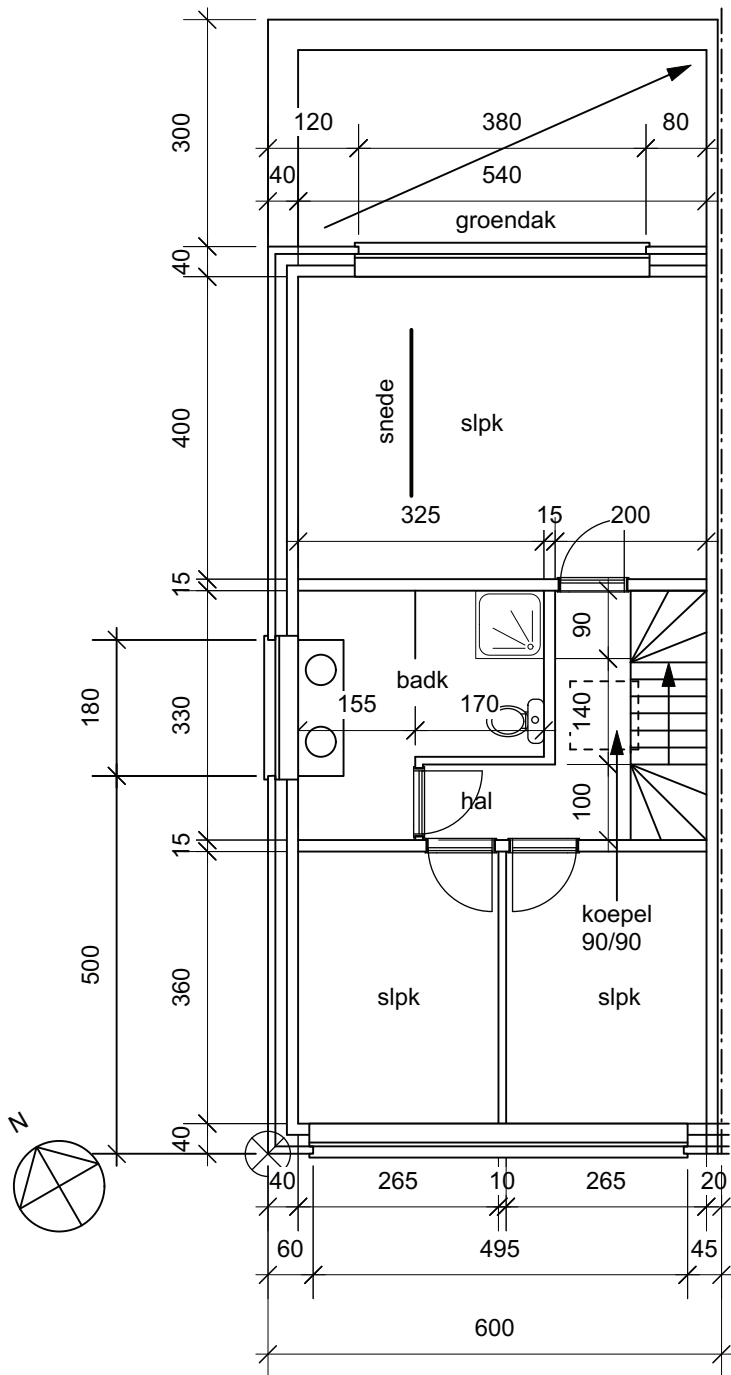
1 verdieping lot 1 1/100
